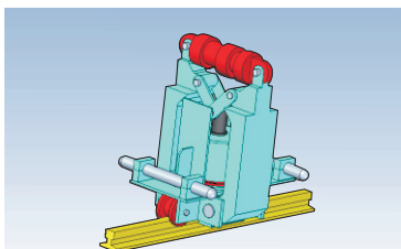
Rail Clamp
