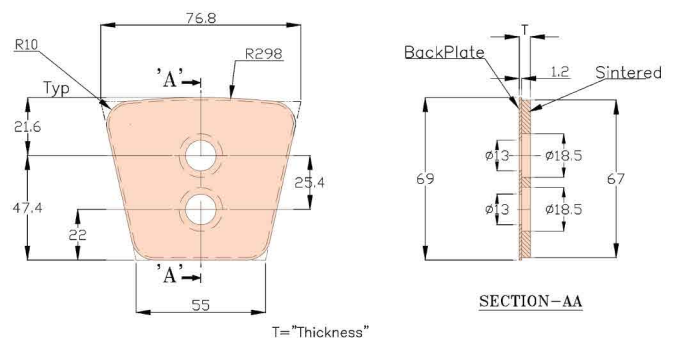
CLUTCH BUTTON
